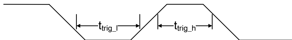
Figure 2-7 Hardware trigger timing
