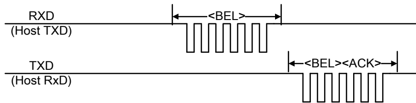
Figure 2-8 Beep timing
