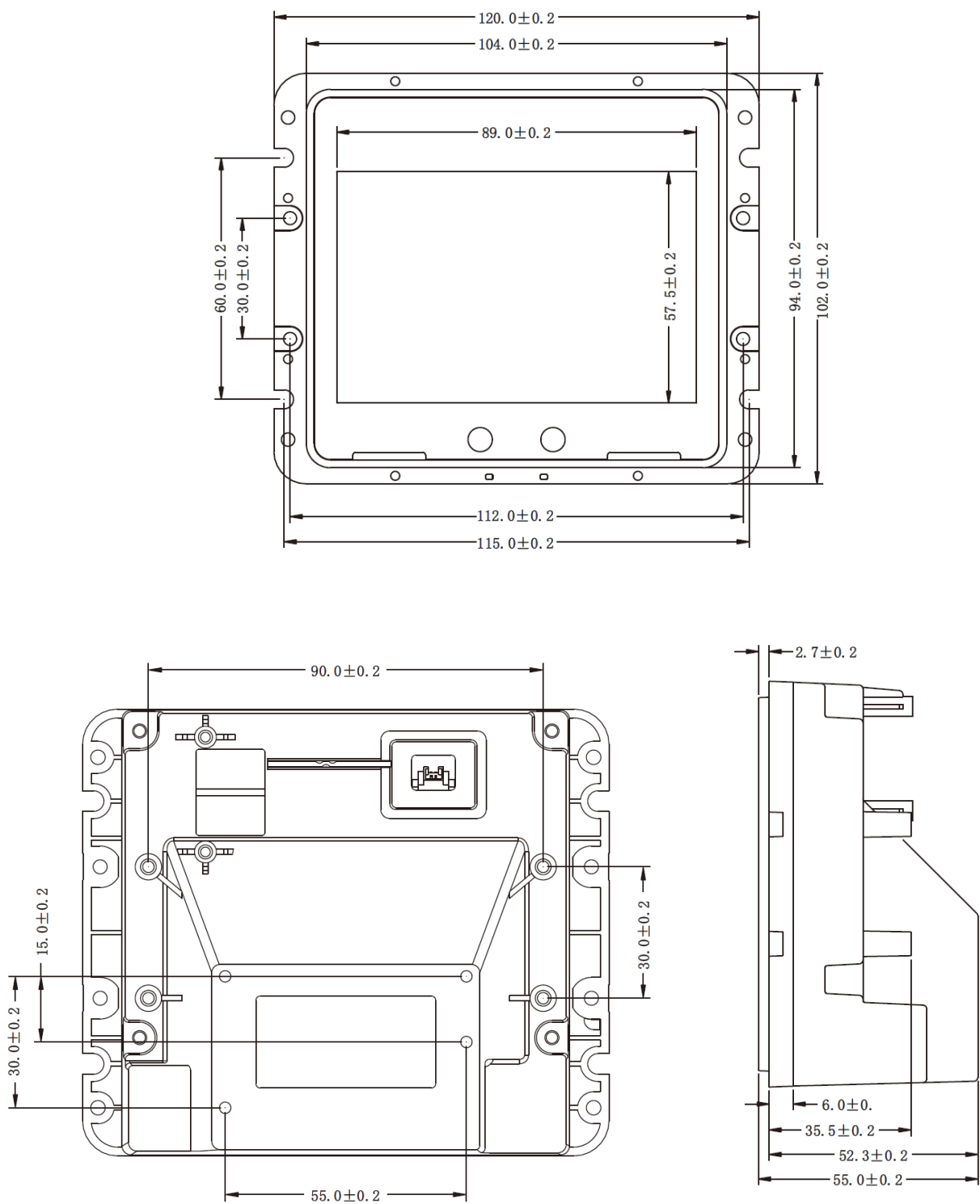
Figure 2-2 Dimensions
