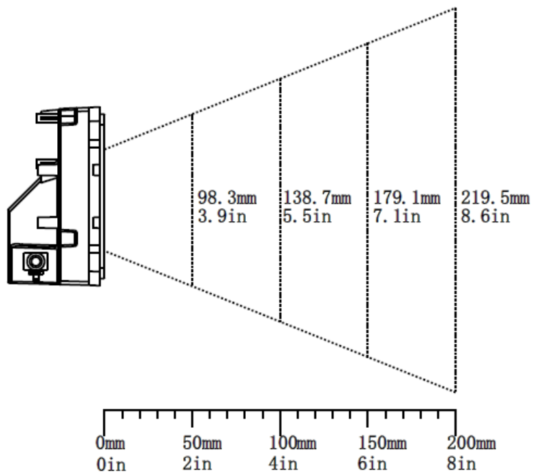
Figure 2-6 Field of view – Vertical
